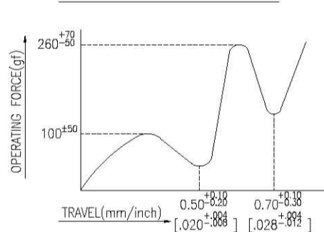
OPERATING FORCE - TRAVEL CHART
